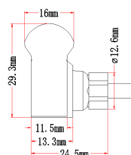
Injection-moulded Middle Connector SF29-IM-MC
