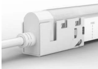
IP65 Clasp Front Connector (Direct) SF29-CL-D
