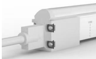
IP68 Screw Front Connector (Direct) SFS29-SC-D
