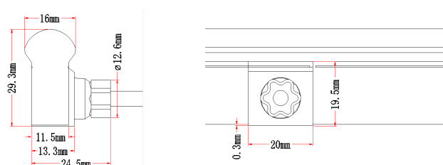
Injection-moulded Middle Connector SFS29-IM-MC
