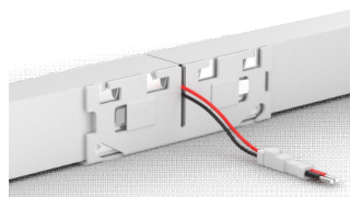
IP65 Seamless Power T-Feed SFS29-CL-MTF
