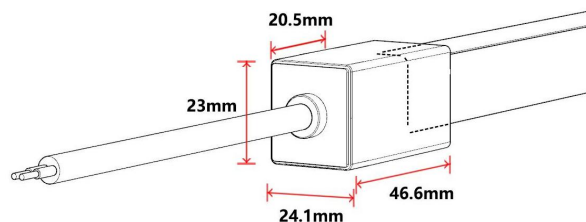
IP67 Sleeve Front Connector (Direct) SFS16-VB-SL-D
