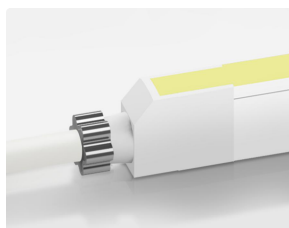
Injection-moulded Front Connector (Direct) SFS09-IM-D
