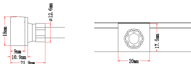
Injection-moulded Middle Connector SF09-IM-MC
