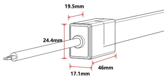
IP67 Sleeve Front Connector (Direct) SF09-SL-D
