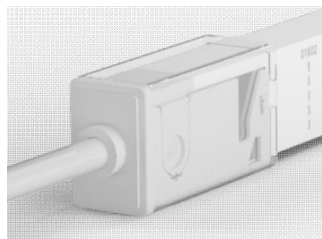
IP67 Sleeve Front Connector (Direct) SF09-SL-D
